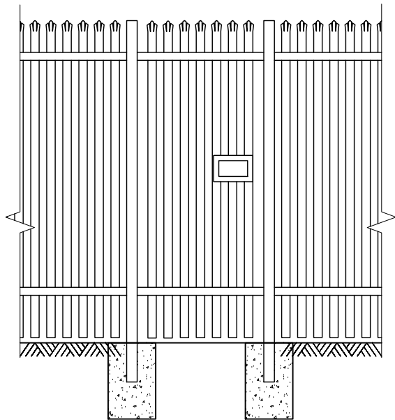
TYPICAL ELEVATION (PEDESTRIAN GATE)
